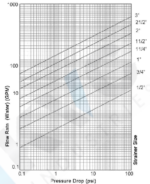
Flow Characteristics of Water in Y-Strainer
